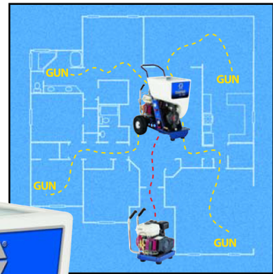
Put the compressor where you'd like it, place the sprayer where you need it.
